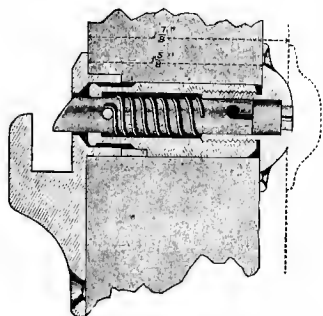
Fig. 4022. KIRBY'S SEAT-LOCK FOR WOOD SEAT-ENDS.
